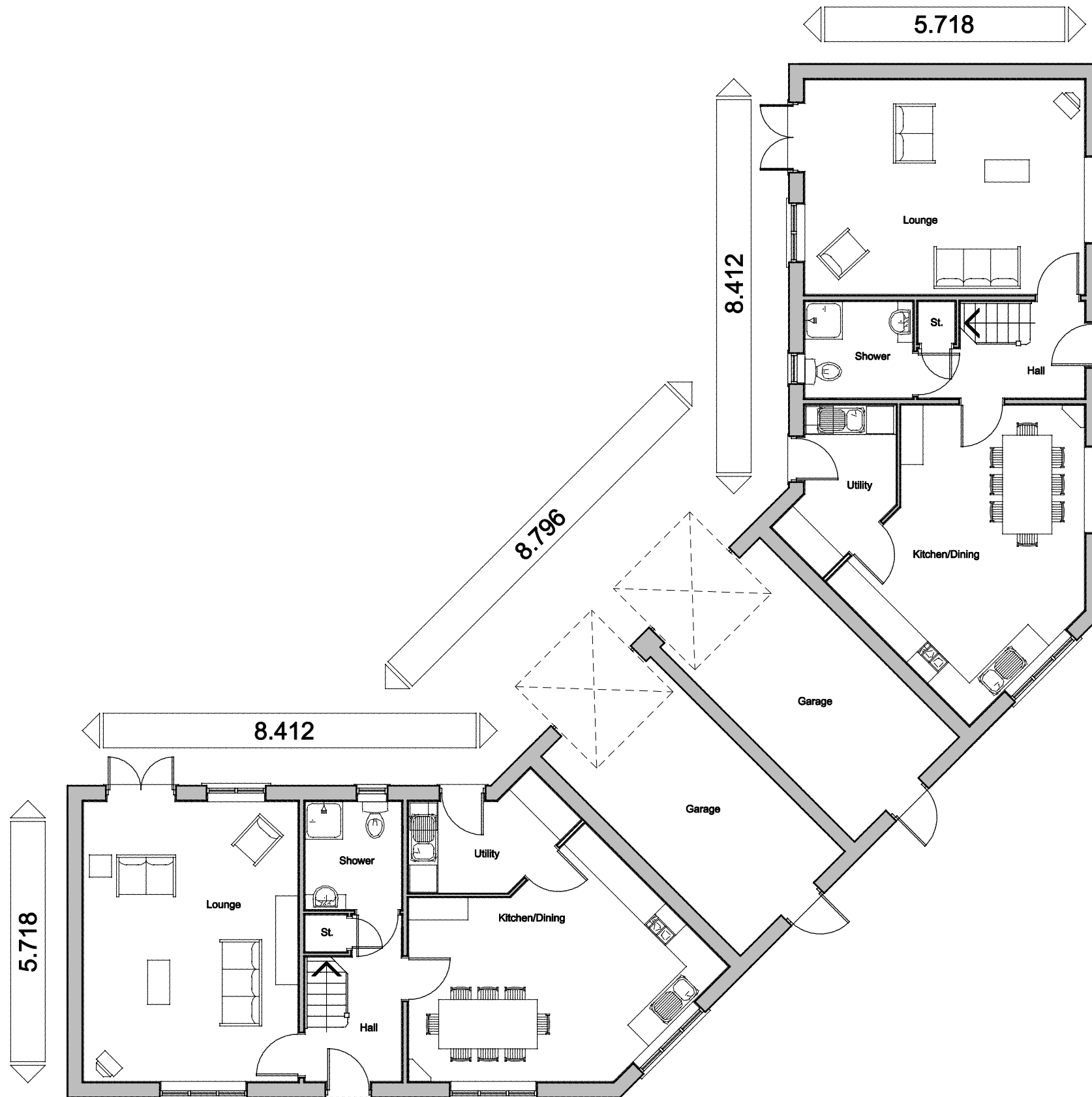
Ground Floor Plan Floor Area - 147.4 sqm 1587 sqft
